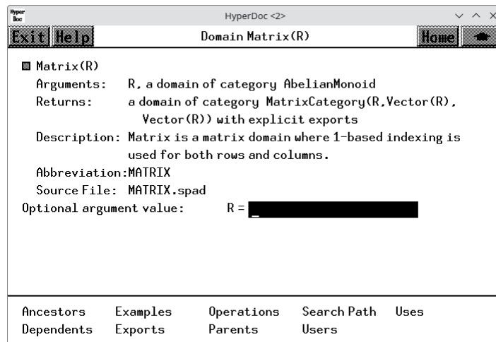
Figure 14.7: Constructor page for Matrix .
