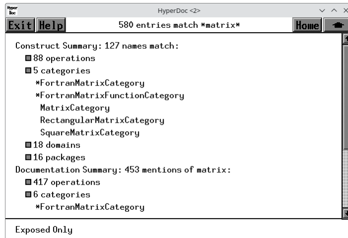
Figure 14.6: Table summarizing complete search for pattern *matrix* .
