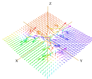
Complex Vector Field
