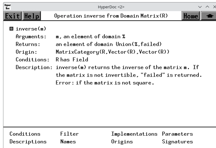
Figure 14.13: Operation inverse from Matrix .
