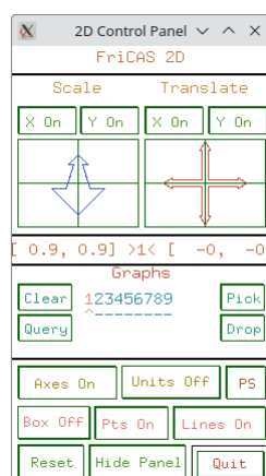
Figure 7.2: Two-dimensional control-panel.
