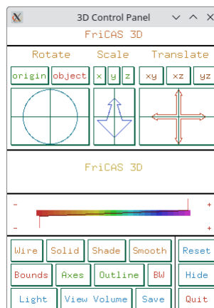
Figure 7.3: Three-dimensional control-panel.
