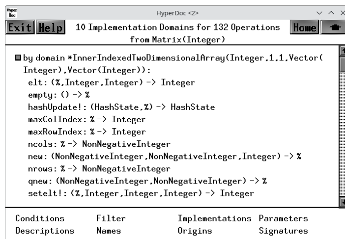
Figure 14.15: Implementation domains for Matrix .
