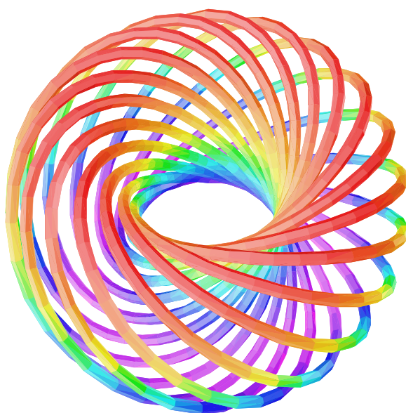
Figure 7.1: Torus knot of type (15,17).
