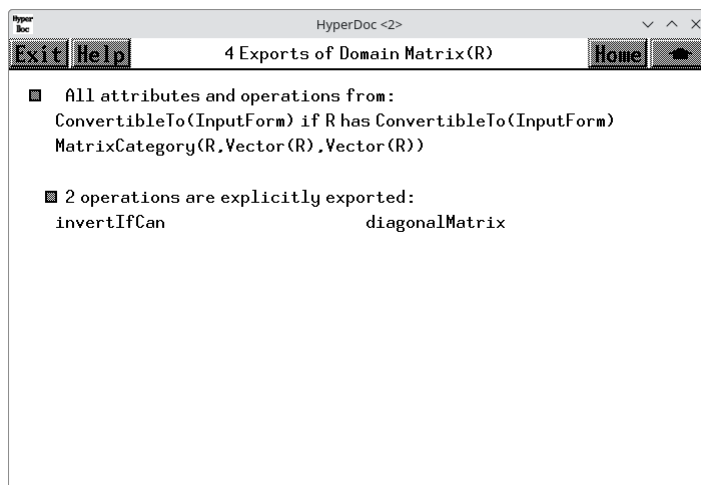
Figure 14.12: Exports of Matrix .
