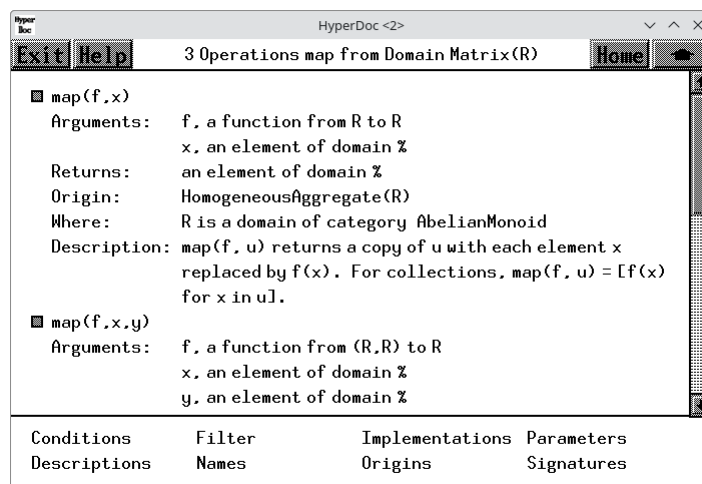
Figure 14.14: Operations map from Matrix .
