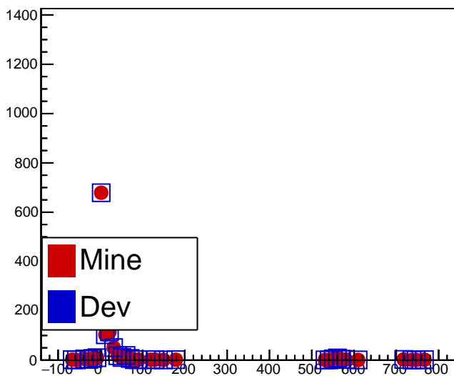
fTime
