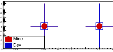
fIndexFwdTracks_MatchMCHTrack
