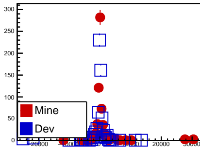
fTPCDCAZ
