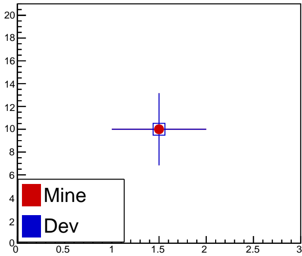
fIndexFwdTracks
