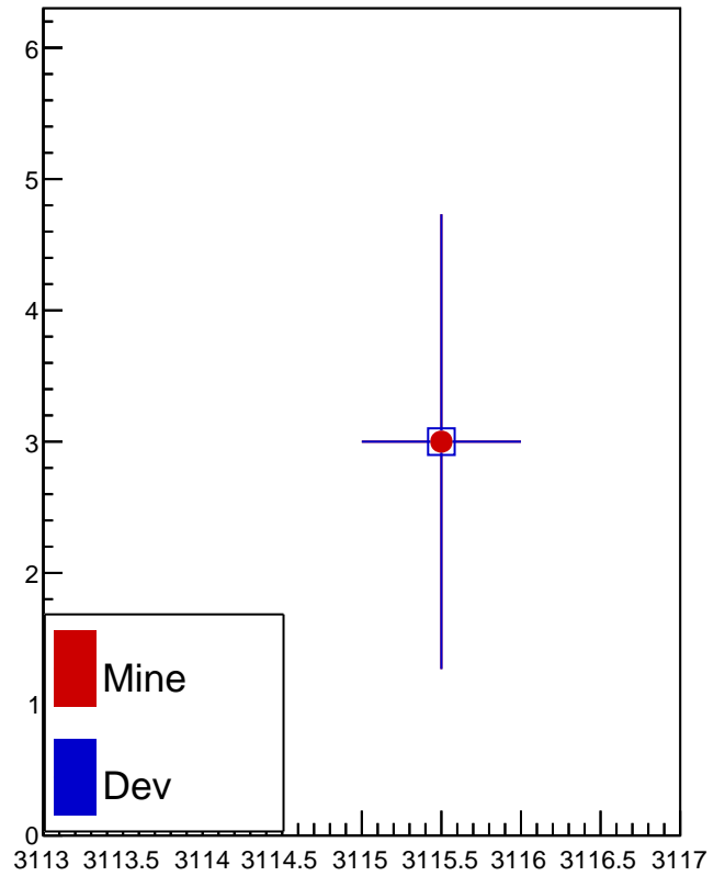
fIndexTracks_0
