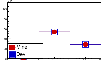
fIndexArray_Mothers_size
