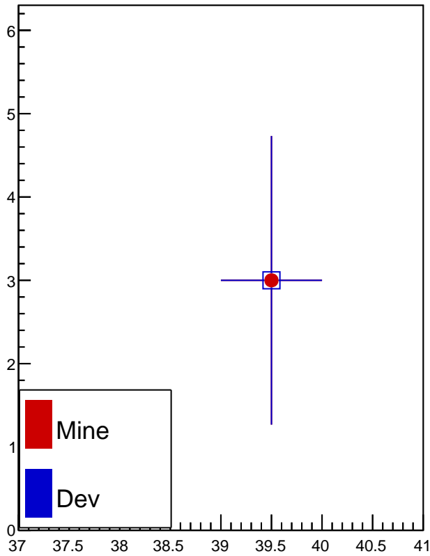
fIndexCollisions
