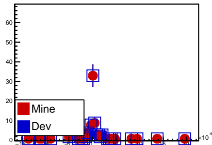
fCovYZ
