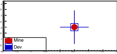
fMIDBoards
