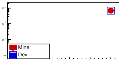
fTrackTime
