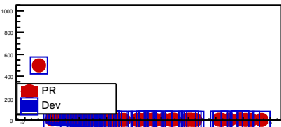
fChi2MatchMCHMID
