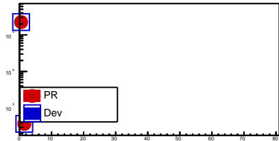
fTPCNClisFindableMinusFound
