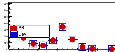
fNClusters
