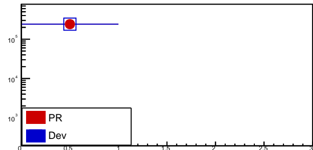
fTrackType
