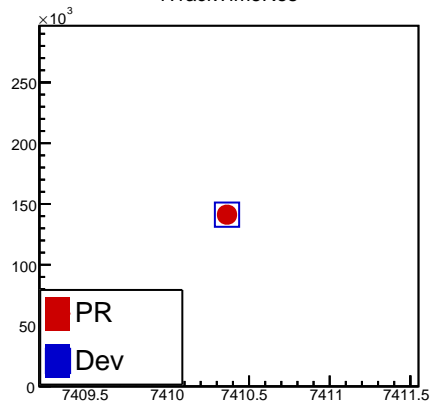
fTrackTimeRes
