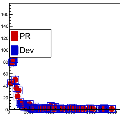
fHMPIDQMip
