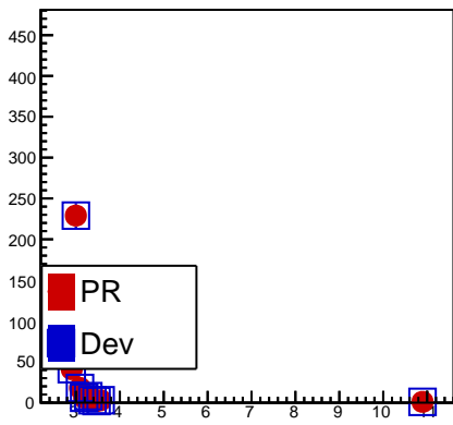
fH3Lmass
