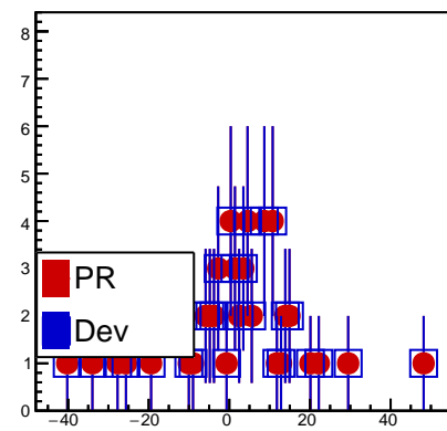
fDecayZ
