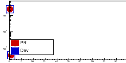
fTPCNClFindableMinusFound
