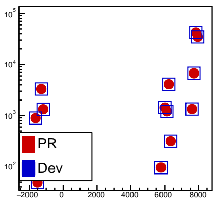
fTrackTime
