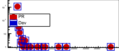
fChi2MatchMCHMFT
