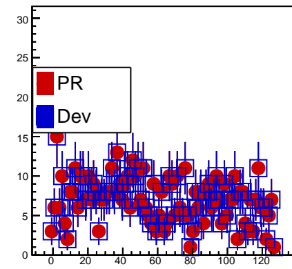
fHMPIDYTrack
