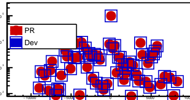
fTrackTime
