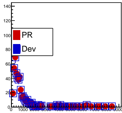
fHMPIDQMip
