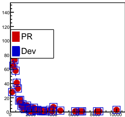
fHMPIDQMip
