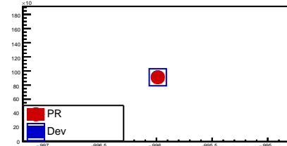
fITSCh2NCI
