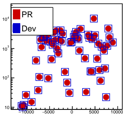
fTrackTime
