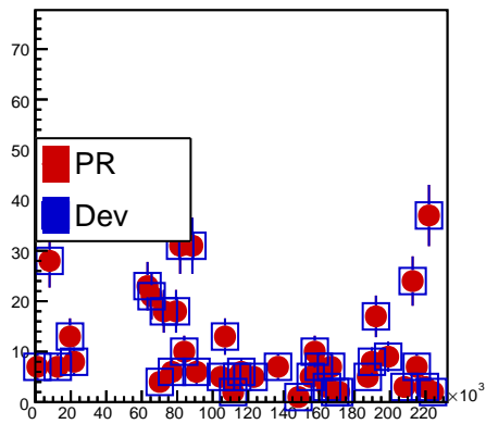
fIndexTracks
