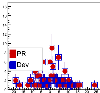
fDecayX
