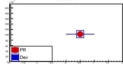
fTSClusterSizes
