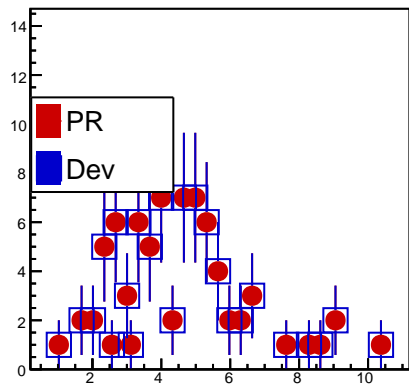
fITSclsSize
