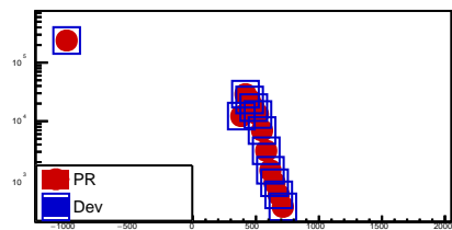
fLength
