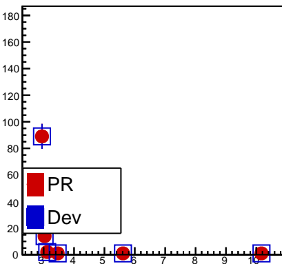
fH3Lmass
