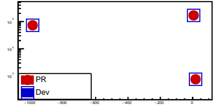
fITSCh2NCI
