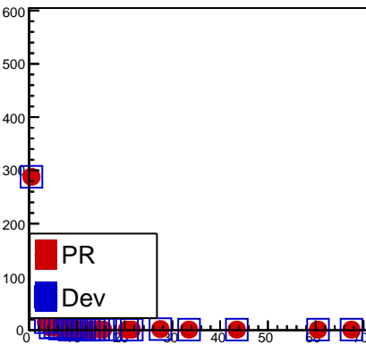
fHMPIDNPhotons
