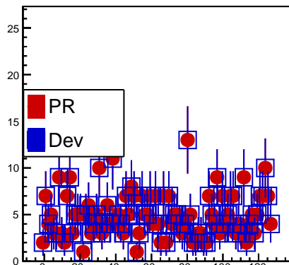
fHMPIDYTrack
