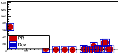
fTrackTimeRes
