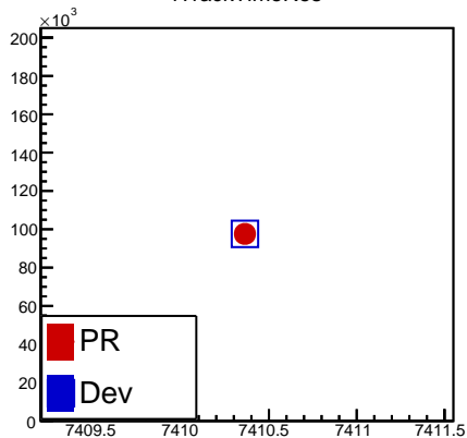
fTrackTimeRes
