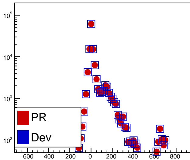
fTime
