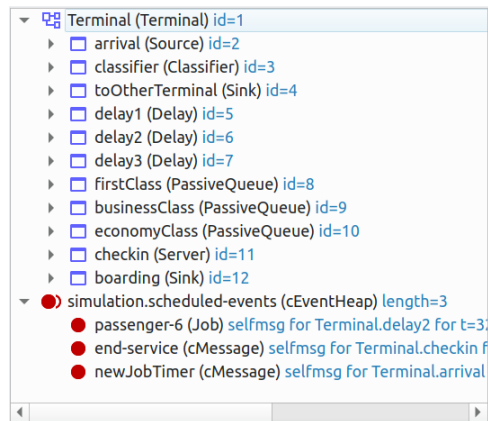
Fig. 7.6: The object tree
