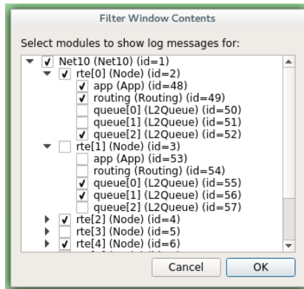
Fig. 7.18: The log filter dialog
