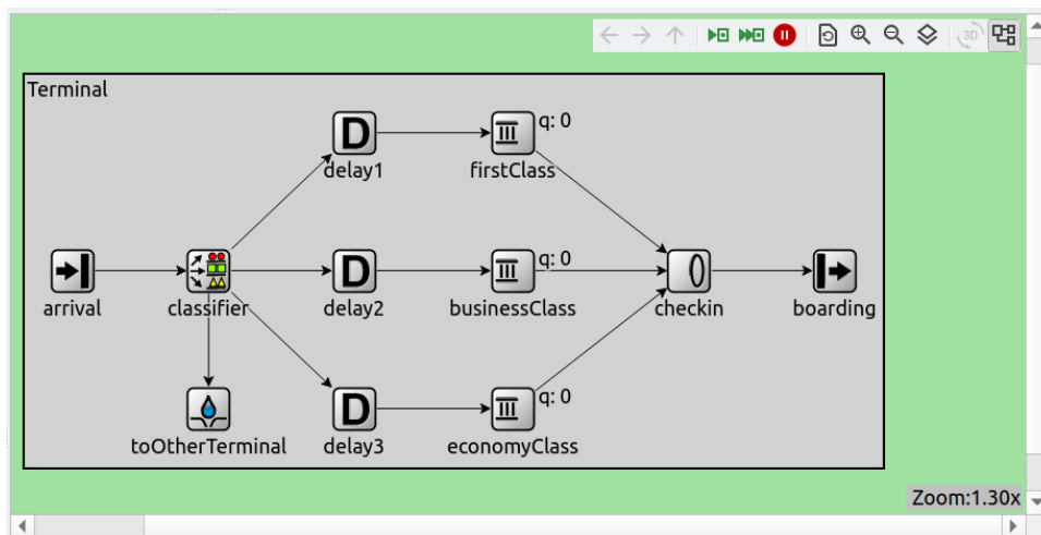
Fig. 7.11: The network display
