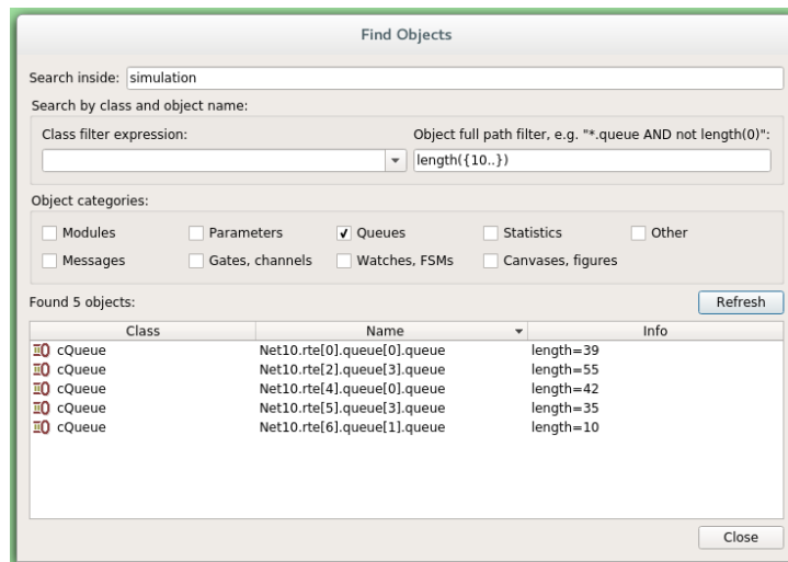
Fig. 7.26: Using the Find/Inspect Objects dialog to find long queues
