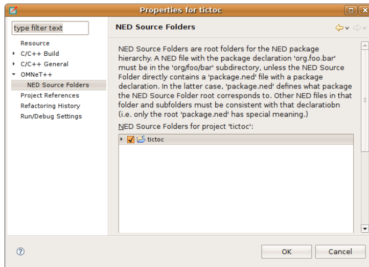
Fig. 2.2: Specifying the folder where NED files will be stored
