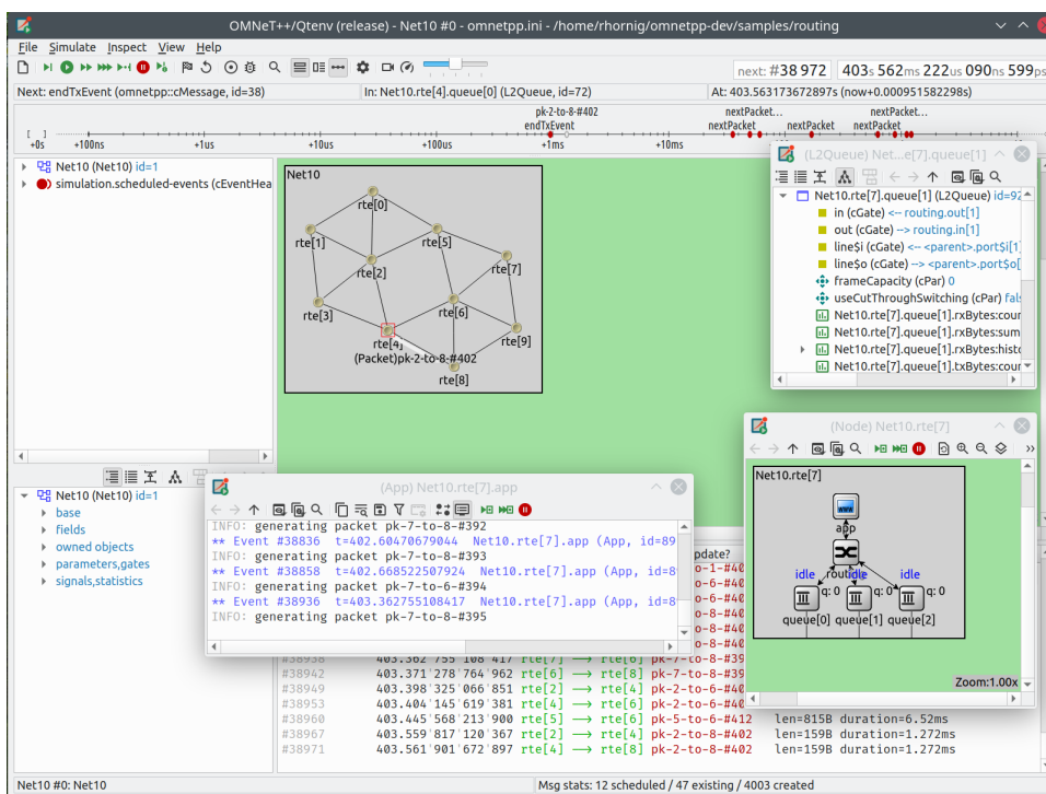
Fig. 7.23: Qtenv with several floating inspectors open
