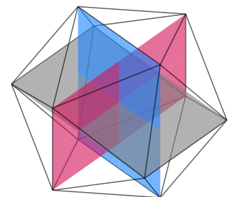
FIGURE 11.1: Icosahedron with an inscribed true cross
