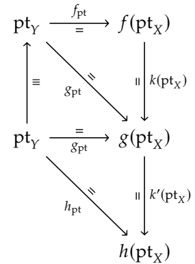
FIGURE 13.1: Path for (k' \cdot_{\text{ptw}} k) .
