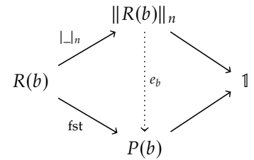
FIGURE 3.15: Taking summands for b : B in Figure 3.14.
